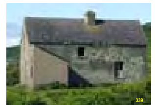
Additive and recessive porch forms - providing an iconic focal point of arrival - the porch should not dominate the elevation but contribute to the overall composition.
